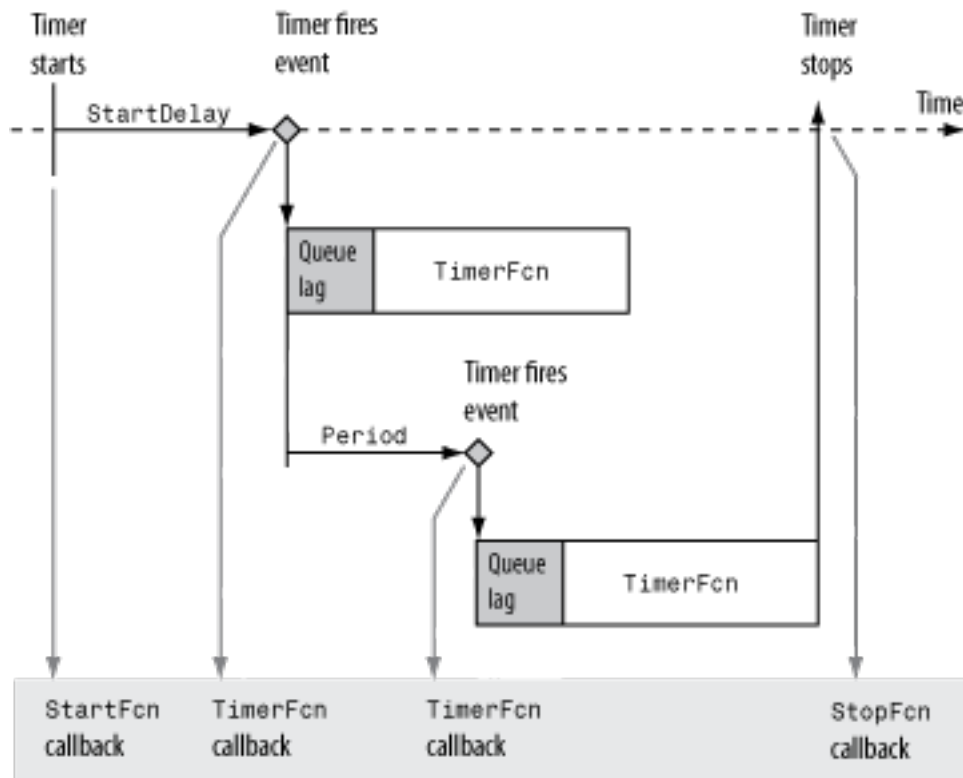
Timer Object Events and Related Callback Function
